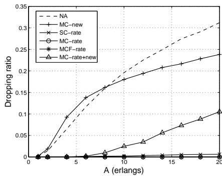
(c) Dropping ratio (100%)
