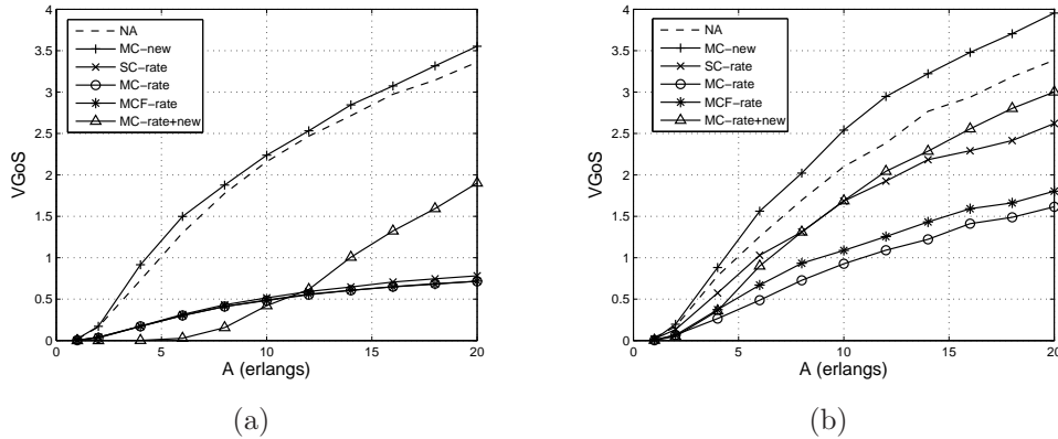
Figure 4: VGoS vs. Offered Traffic for (a) 100% node participation, (b) 40% node participation
