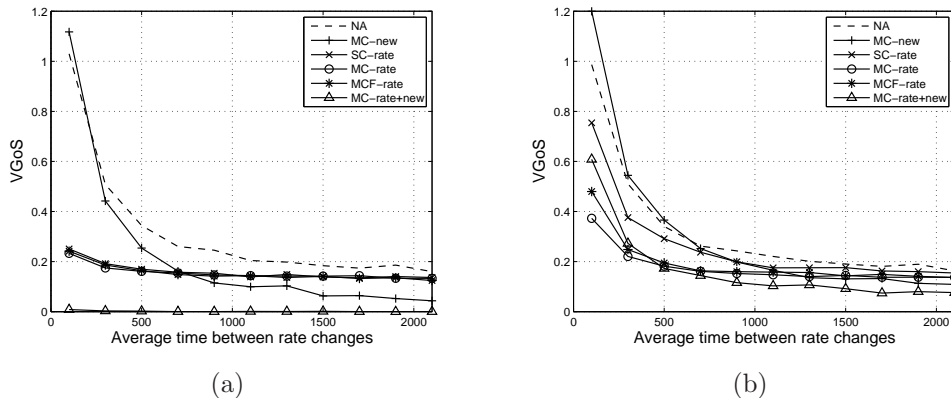
Figure 5: VGoS-factor vs. frequency of rate changes at 5 Erlangs with (a) 100% node participation, (b) 40% node participation
