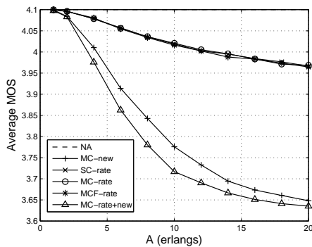
(e) Average MOS (100%)
