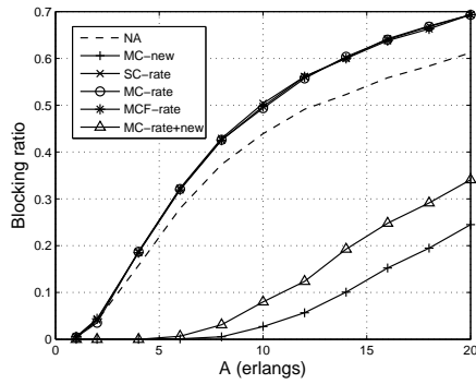
(a) Blocking ratio (100%)
