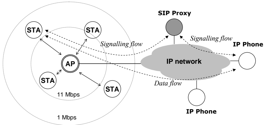
Figure 2: A VoIP WLAN Hotspot scenario
