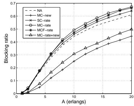
(b) Blocking ratio (40%)
